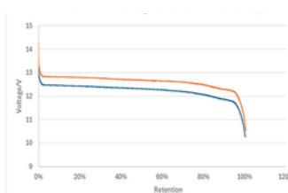
Discharge Curve at Different Rates @ 25°C
