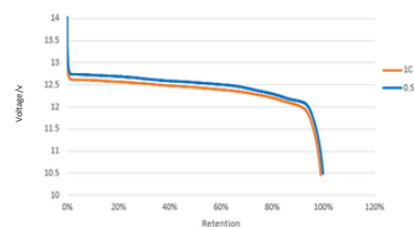
Discharge Curve at Different Rates @ 25°C
