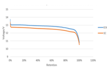
Discharge Curve at Different Rates @ 25°C
