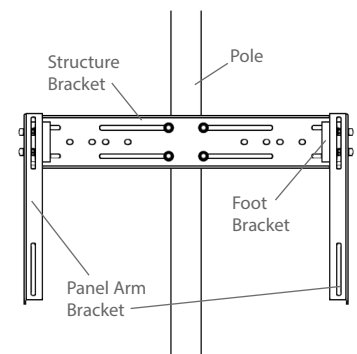
Figure 3: Pole Mount Front View
