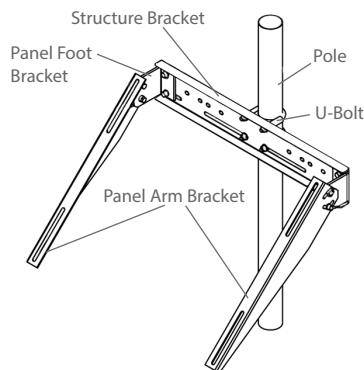
Figure 2: Pole Mounting Quartering View
