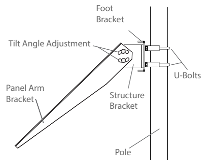
Figure 1: Pole Mount Side View
